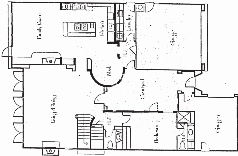
PLAN 1 APPROXIMATELY 3090 SQ. FT. PRELIMINARY FLOOR PLANS AS OF 10/24/98
